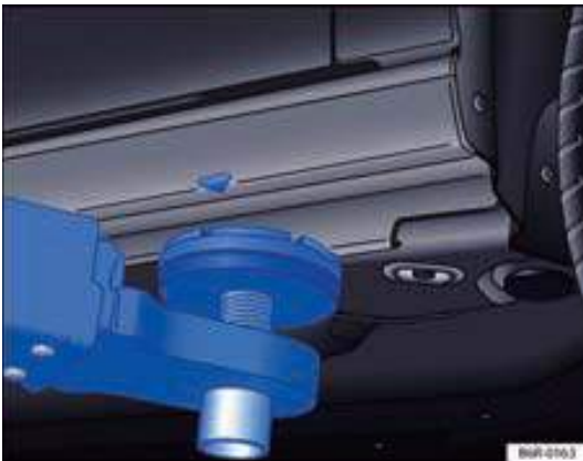
Fig. 97 Front jacking points to lift the vehicle with a lifting platform or car jack.
