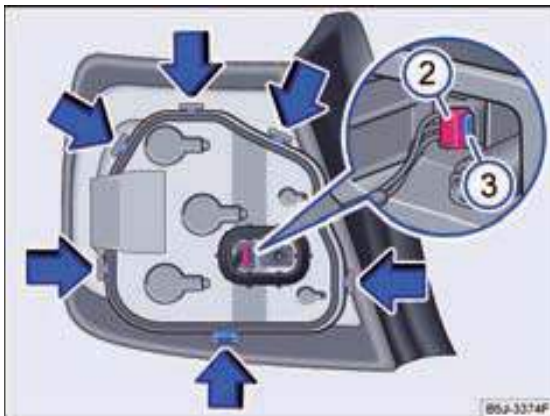
Fig. 121 Tail light assembly: Removing the bulb housing.
