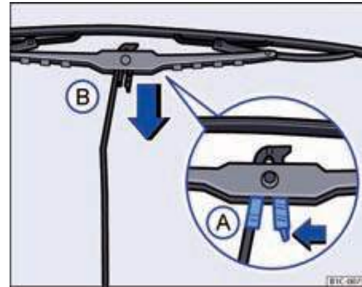
Fig. 88 Replacing the windscreen wiper blades.
