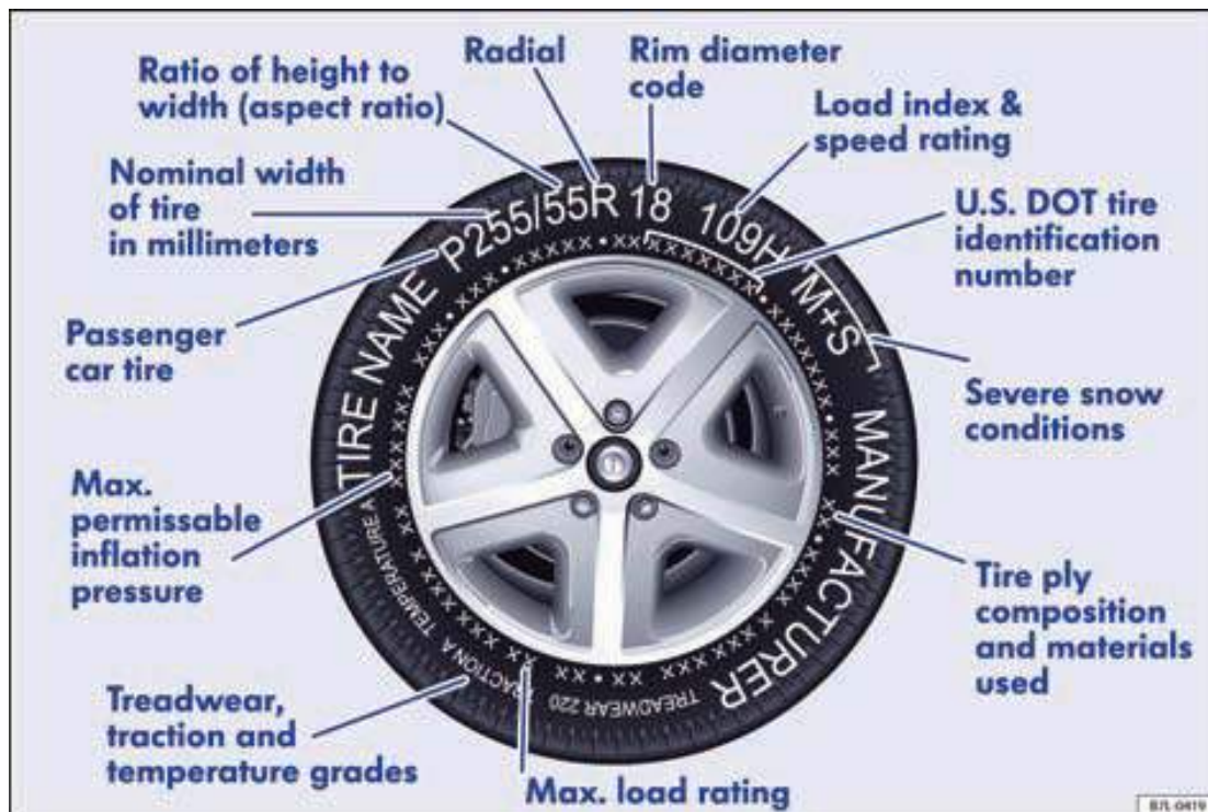
Fig. 96 International tyre inscription.
