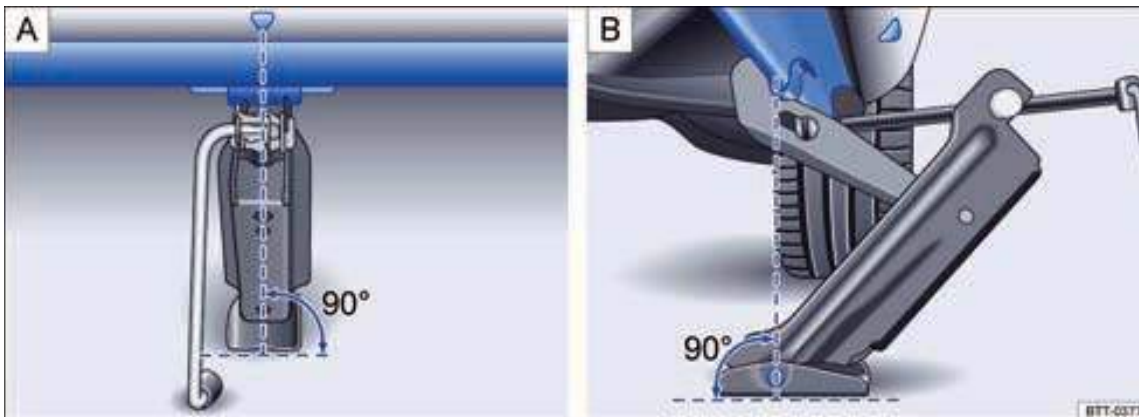
Fig. 112 Jack applied at rear left side of the vehicle.
